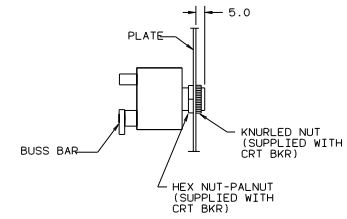
SECTION U-U
