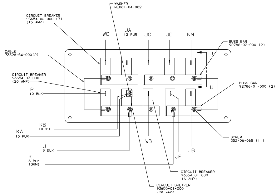
CIRCUIT BREAKER (I) (BACK VIEW)
