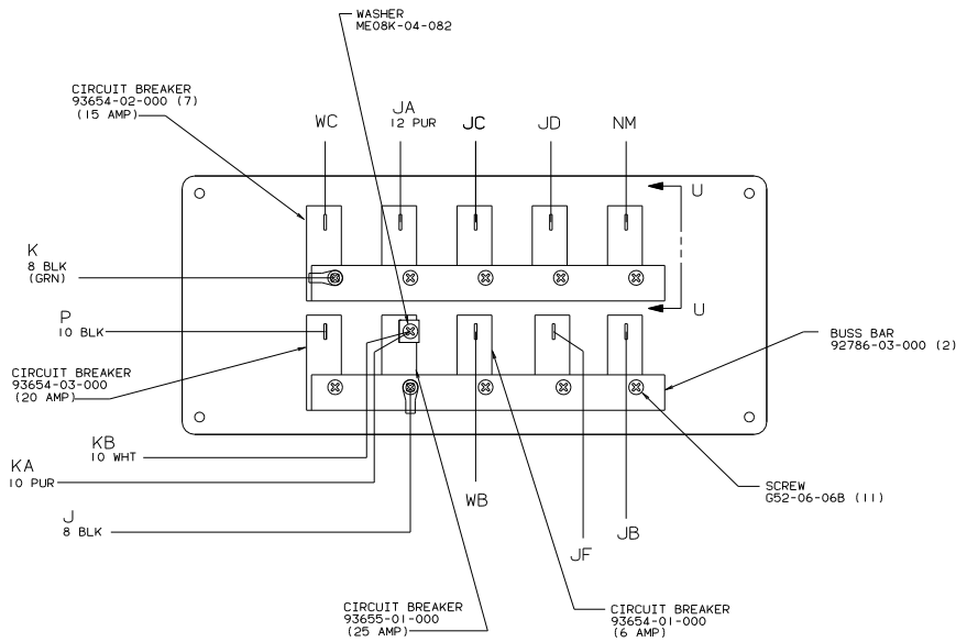
CIRCUIT BREAKER (W) (BACK VIEW)
