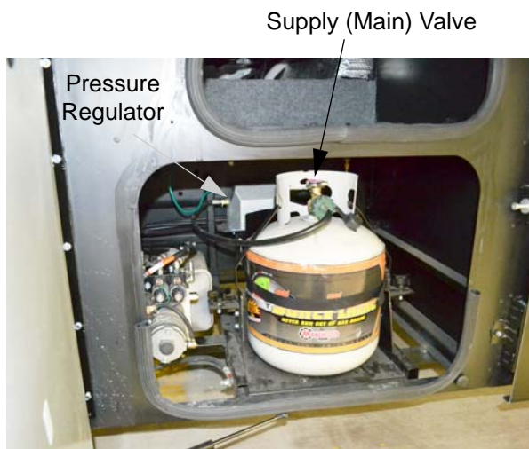
-Typical View
