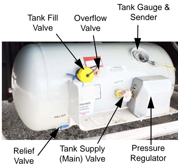
Propane Tank Features -Typical View
