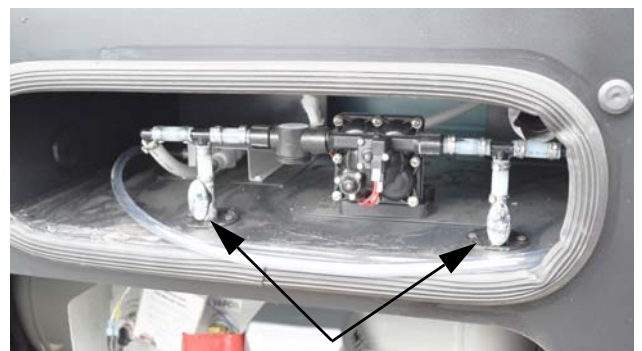
Waterline Drain Valves (Located in driver side compartment) -Typical installation shown
