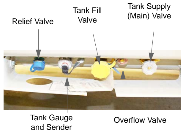
Propane Tank Features (Located on driver side of coach) Remove cover to access. -Typical View
