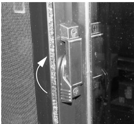
Slider Window Latch (Lift latch UP and slide window open) -Typical View
