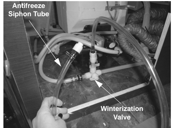
Antifreeze Siphon Tube and Winterization Valve
