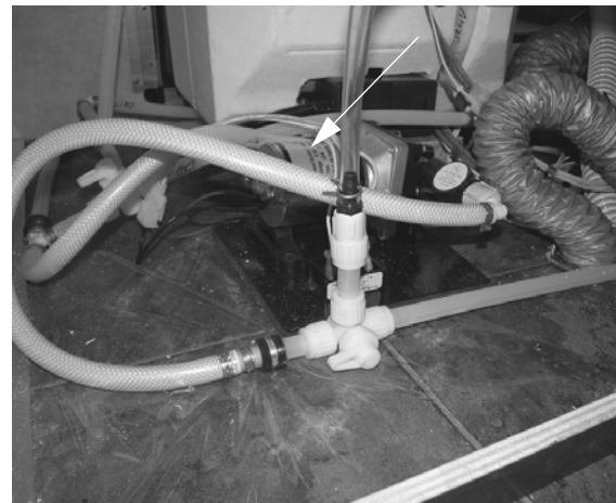
Water Pump (Model 524V)
