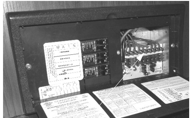
House 12-Volt Fuses (Located on right-hand side of Power Converter) -Typical View
