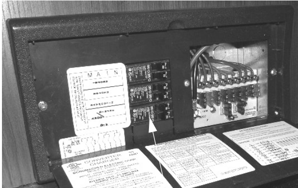
120-Volt Circuit Breakers -Typical View
