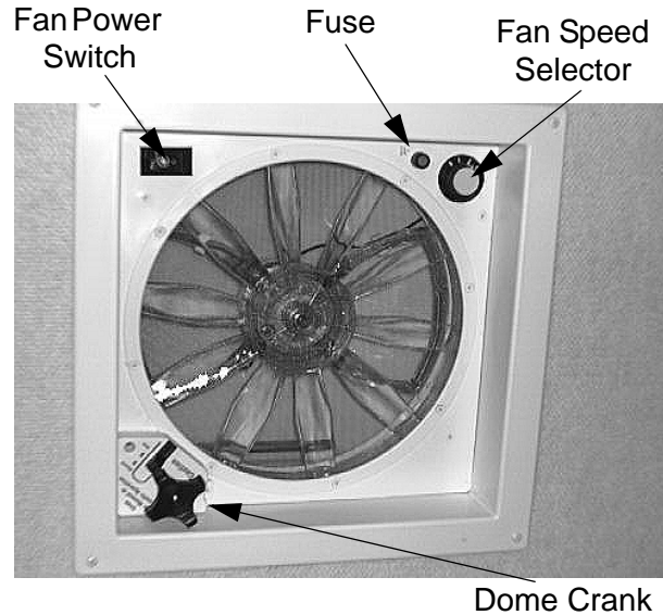
Power Ventilator -Typical View
