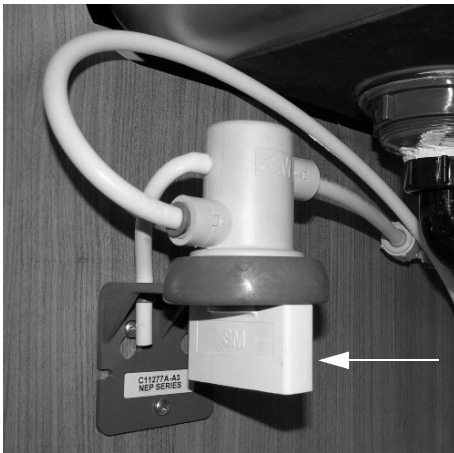
Diverter Plug (installed in filter socket)
