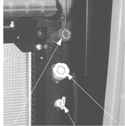
Transmission Fluid Fill/Dipstick Engine Oil Dipstick Engine Oil Fill
