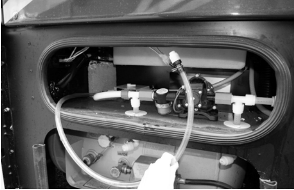
RV Antifreeze Siphon Tube (Located near water pump - second compartment on driver side of coach)
