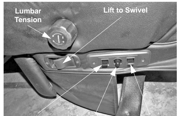
Lumbar Tension Lift to Swivel Hip Area -Up/Down Main Seat Position -Up/Down -Fore/Aft Knee Area -Up/Down
