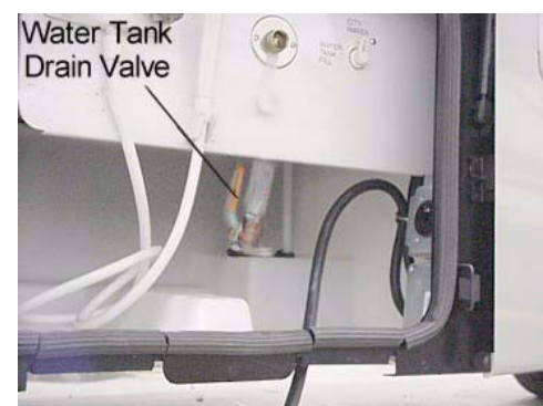
typical installation
