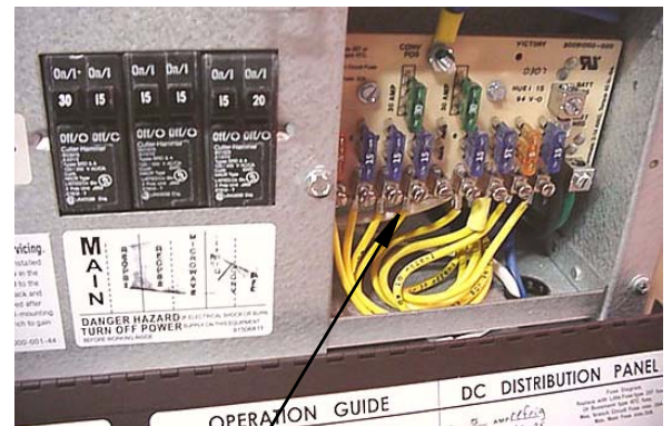
House 12V Fuses (on converter panel) 26' to 30' models
