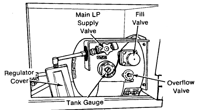
Typical LP Gas System Controls
