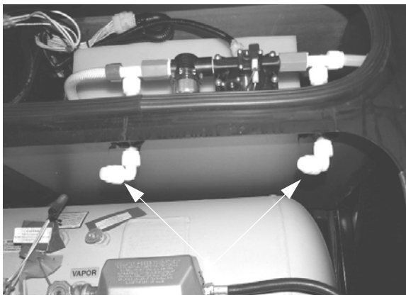
Waterline Drain Valves (Located in driver side compartment) -Typical installation shown
