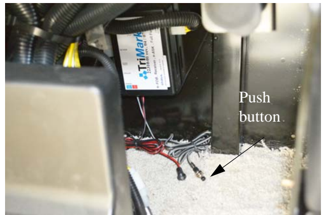
Keyless Entry Control Box (Located below driver side dash) -Typical View
