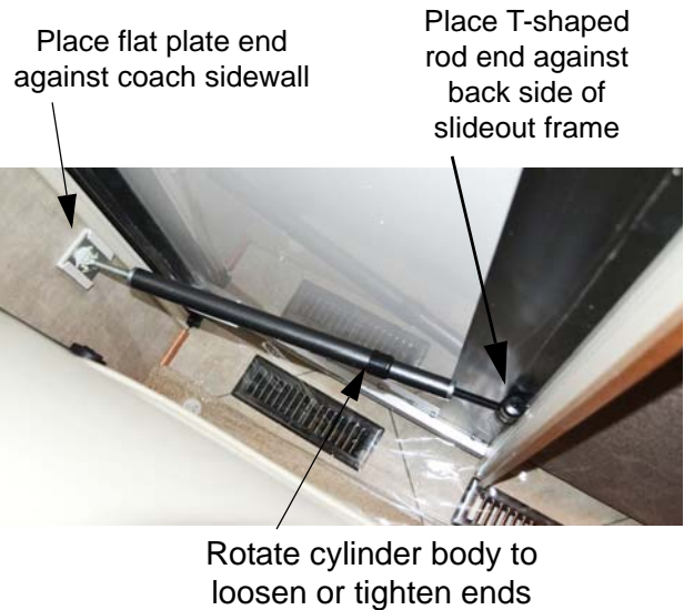
Slideout Room Prop-Lock Rod Typical view of forward end of retracted slideout room. Your model may differ in appearance.
