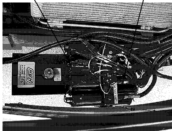
Hydraulic Pump - Slideout/Leveling Systems (top view from hood opening)
