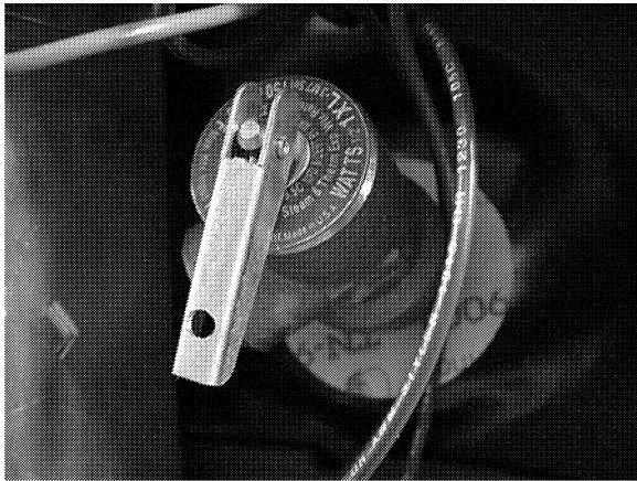
Lift straight out to open P-T valve
