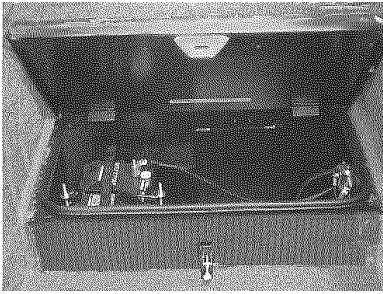
House Battery Storage in Entrance Step Models 27', 29' & 31'
