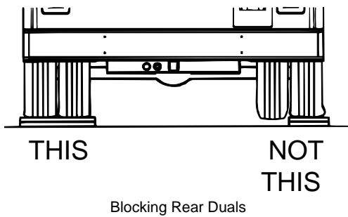
Blocking Rear Duals
