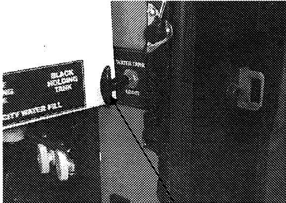
Water Tank Drain Valve - Model 36WL Freightliner Diesel
