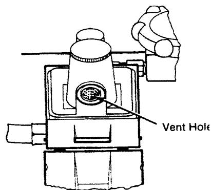
LPG PRESSURE REGULATOR 1R (Typical)
