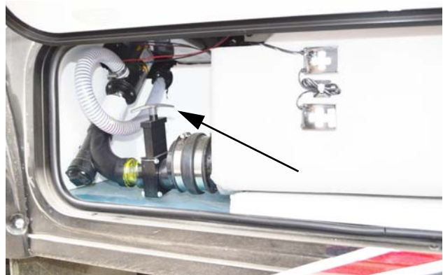
Gray Waste Tank Drain Valve (Located in driver side compartment behind rear wheel)
