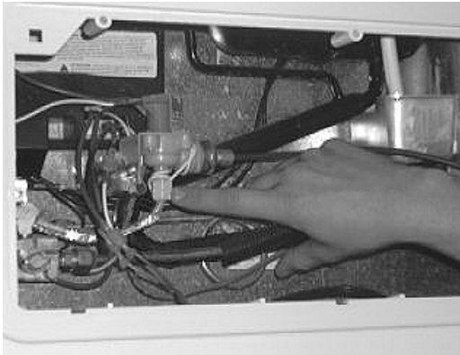
Ice Maker Water Supply Connection -Typical View
