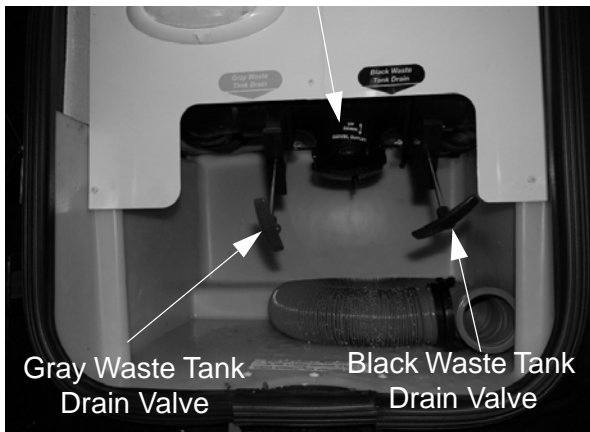
Holding Tank Drain Valves (Located in holding tank compartment) -Typical View
