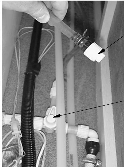
Winterization Valve (See Drain Valve Location chart at end of this section) -Typical View
