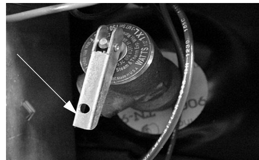
Pressure-Temperature Relief Valve (Lift handle only when water heater is cold) -Typical View
