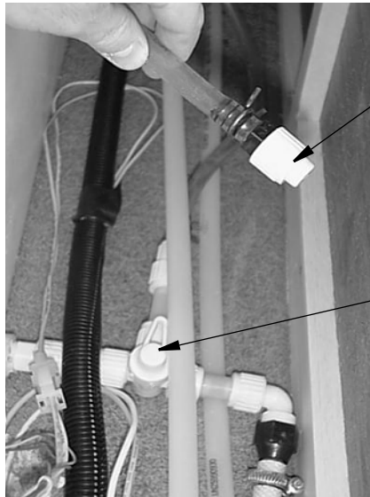
Antifreeze Siphon Tube and Winterization Valve (See Drain Valve Location chart at end of this section) -Typical View
