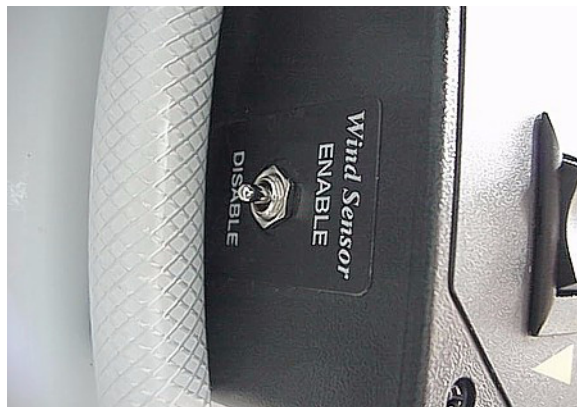
Wind Sensor Control Switch on inboard end of control box.
