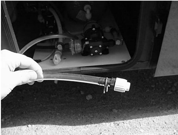
RV Antifreeze Draw Tube in water center or near water pump (insert into container of RV water system antifreeze)
