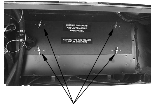
Twist Locks to Remove Cover
